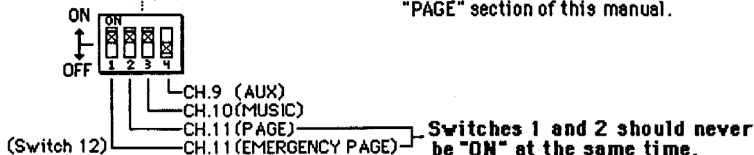
MIX BUS SWITCH FOR INPUTS 9-11
